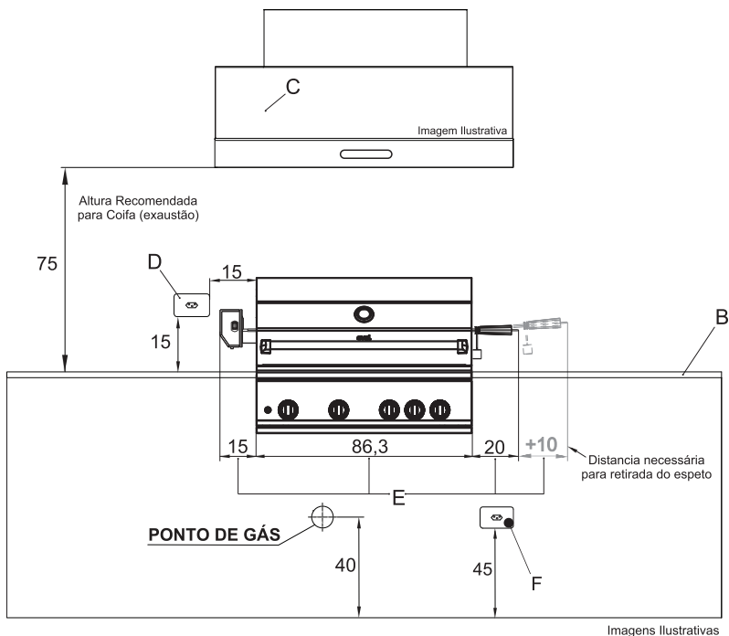
VISTA FRONTAL
